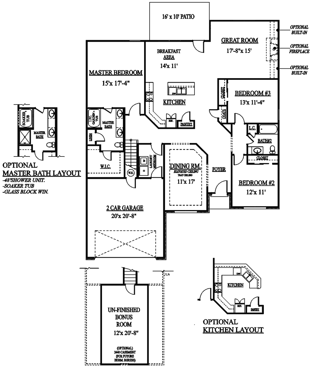
BONUS ROOM LAYOUT -ABOVE GARAGE
