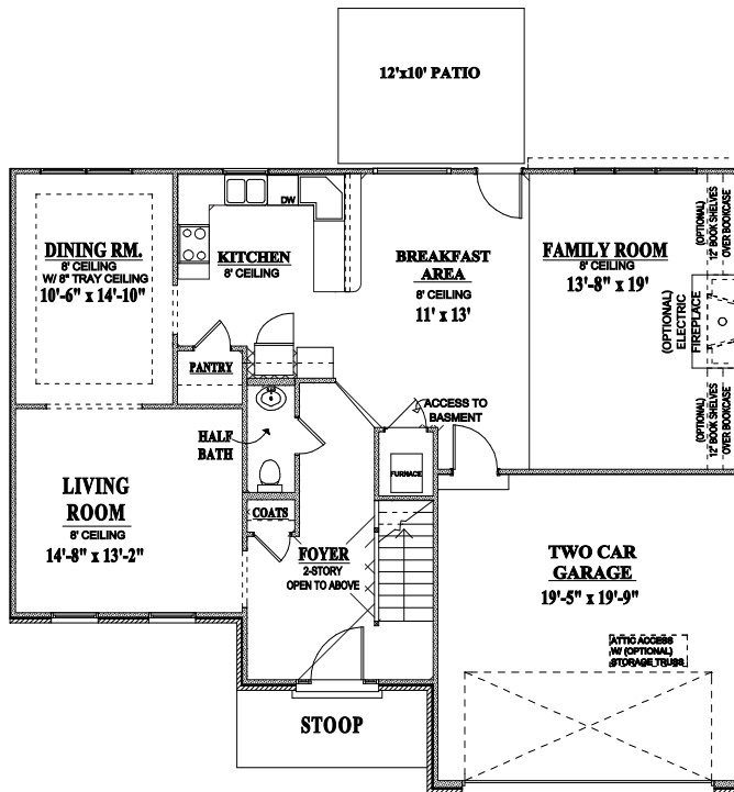
First Floor 1255 Square Feet
