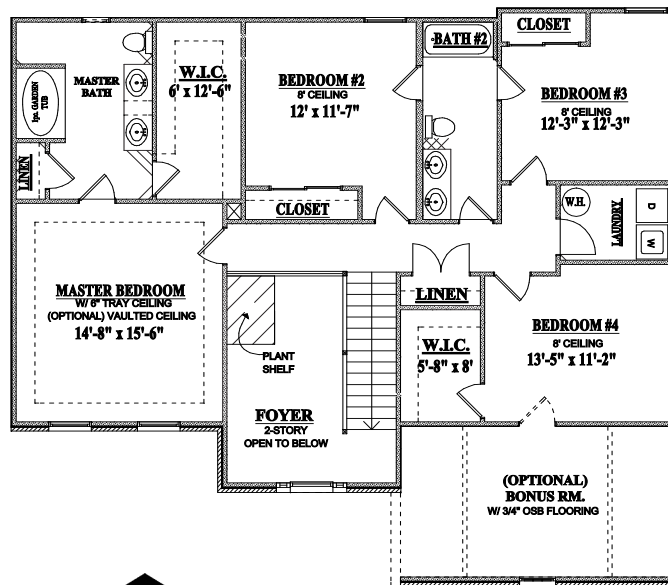
Second Floor 1258 Square Feet
